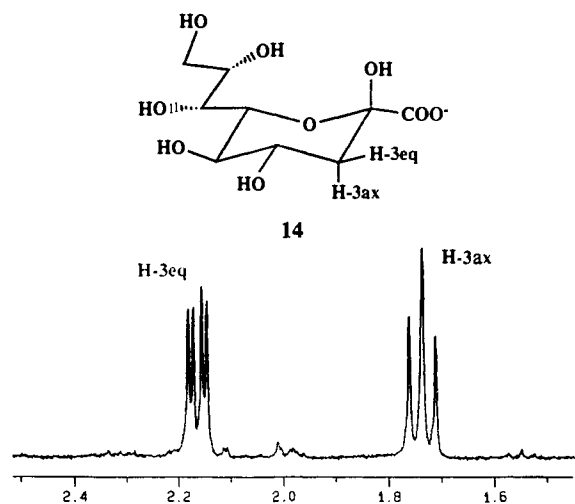
Figure 1. The 1 H NMR spectrum of compound 14 shows the coupling type of H-3ax and H-3eq.
