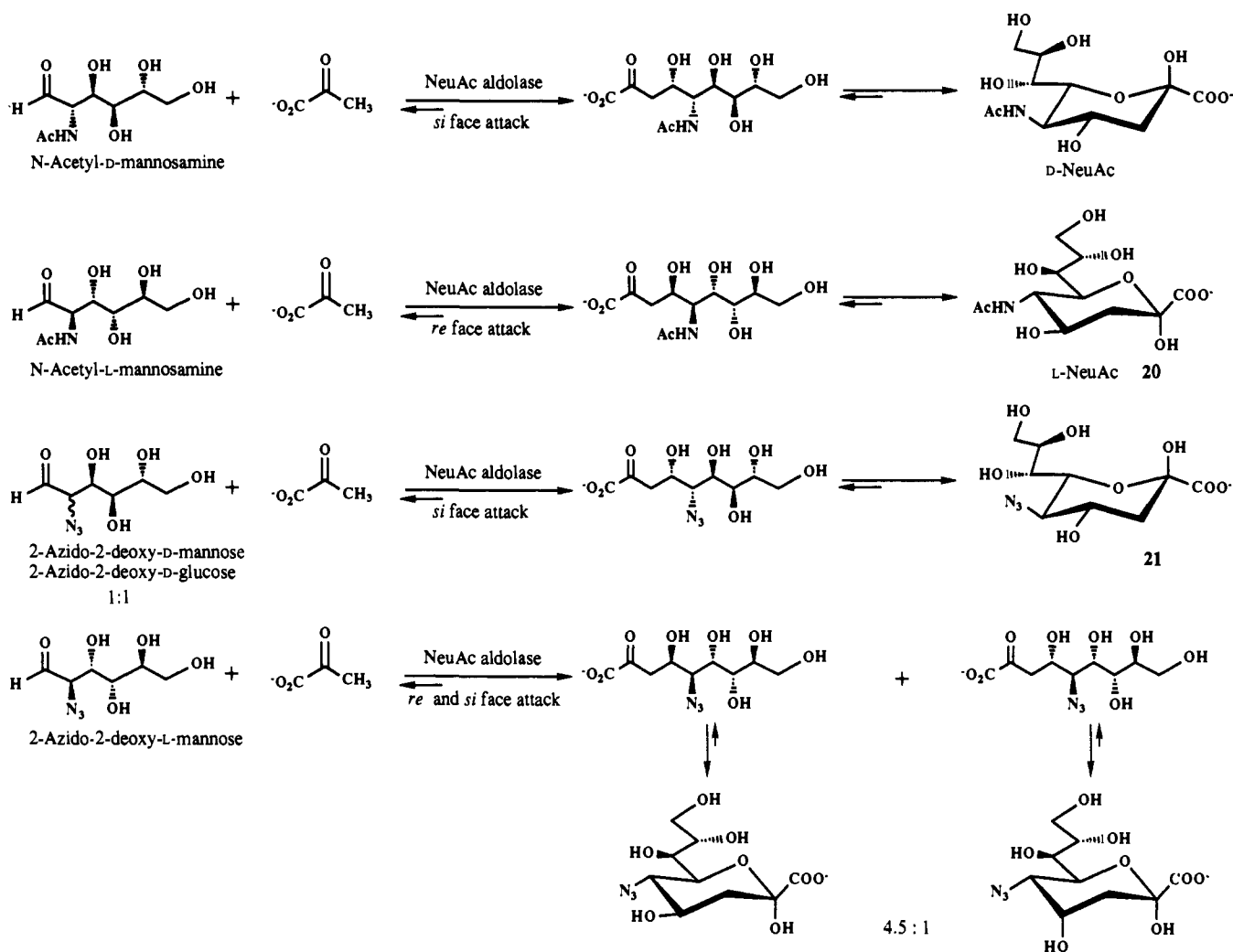
Scheme VI (continued)
